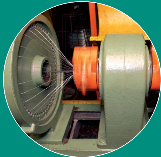
Armouring Process
